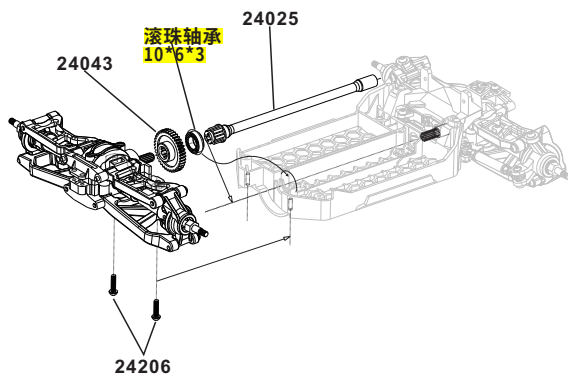
底盘后部套与主轴装配 Rear Chassis Assembly and Main Shaft
