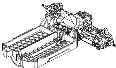
底盘前部套装配 Front Chassis Assembly
