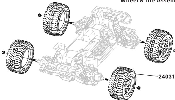
轮胎装配 Wheel & Tire Assembly
