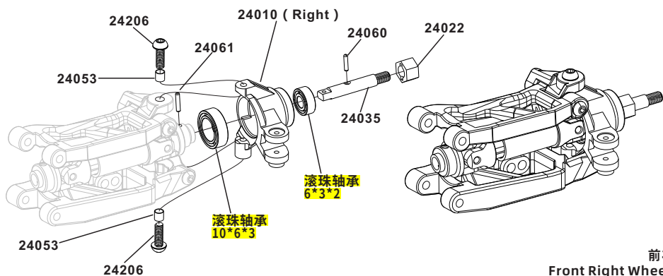
前右摆臂 Front Right Suspension Arm
