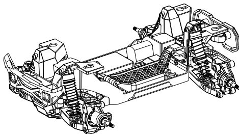
避震器装配 Shock Absorber Assembly
