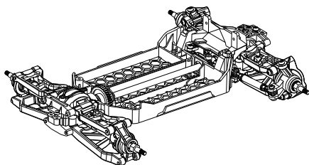
底盘后部套与主轴装配 Rear Chassis Assembly and Main Shaft
